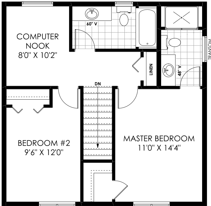
2ND FLOOR PLAN 676 Sq. Ft.
