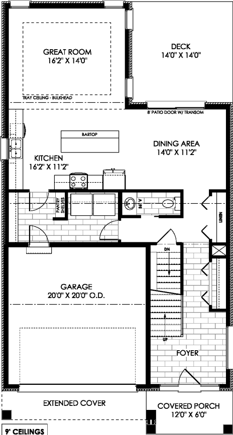
MAIN FLOOR - 1134 SQ. FT.
