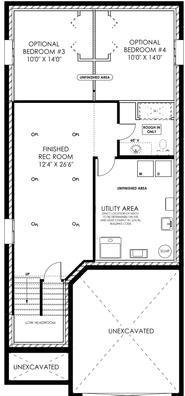
LOWER LEVEL PLAN
